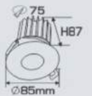
AFC 738 LED 7W 354.000
