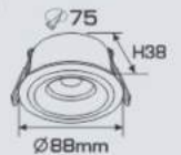
AFC 718 V LED 7W 328.000
