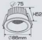
AFC 737 LED 7W 337.000
