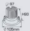
AFC 746 LED 12W 732.000
