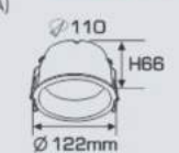
AFC 586 LED 15W 592.000
